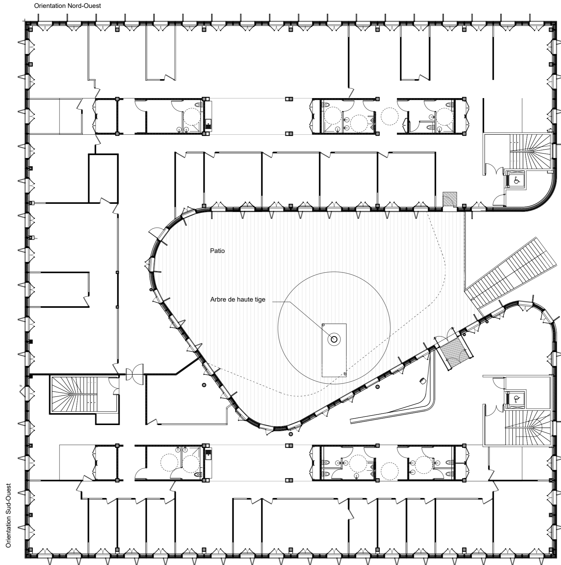
PLAN R+1
