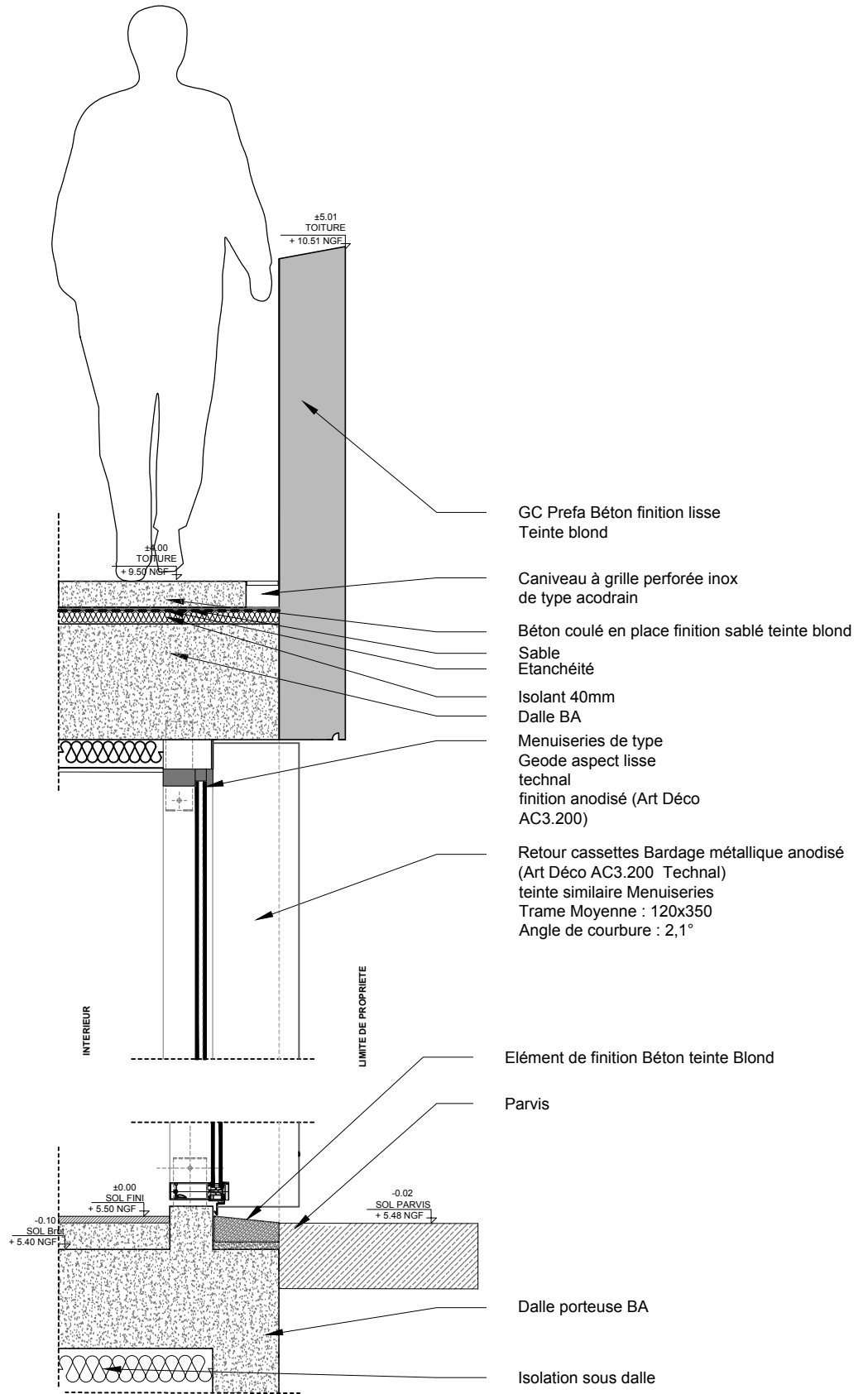
DETAIL COUPE VERTICALE FACADE MUR RIDEAU
