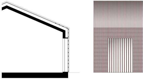
COUPE / FACADE
